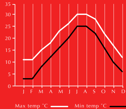
Avg. monthly temperatures in Tokyo
